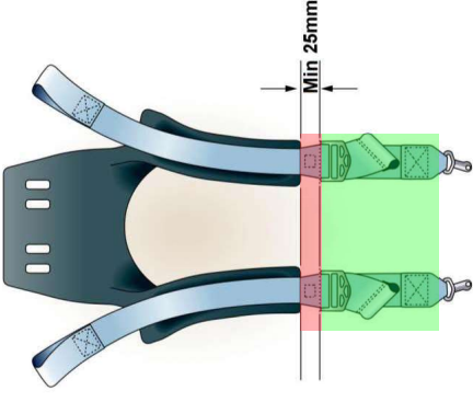
Routing of 2" webbing
